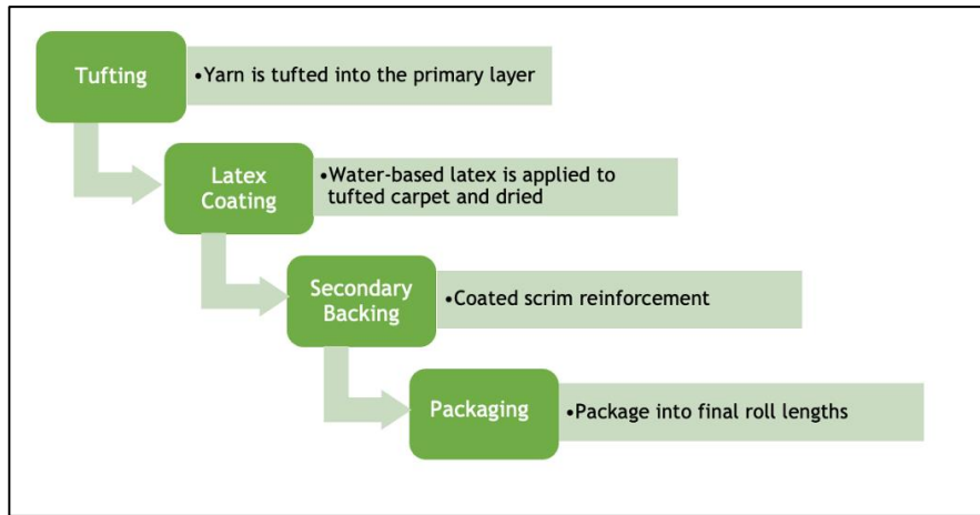
Figure 3: Production process for Milliken Broadloom Carpet
